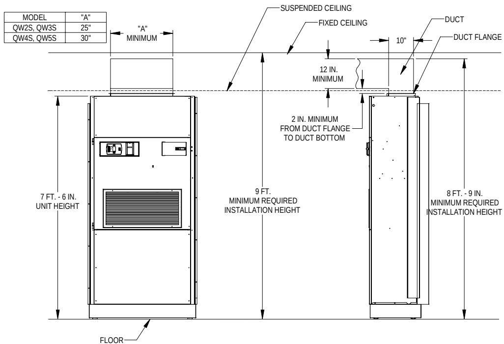
FIGURE 8 Ducted Application
