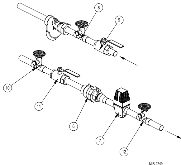
Figure 36 Piping Diagram
