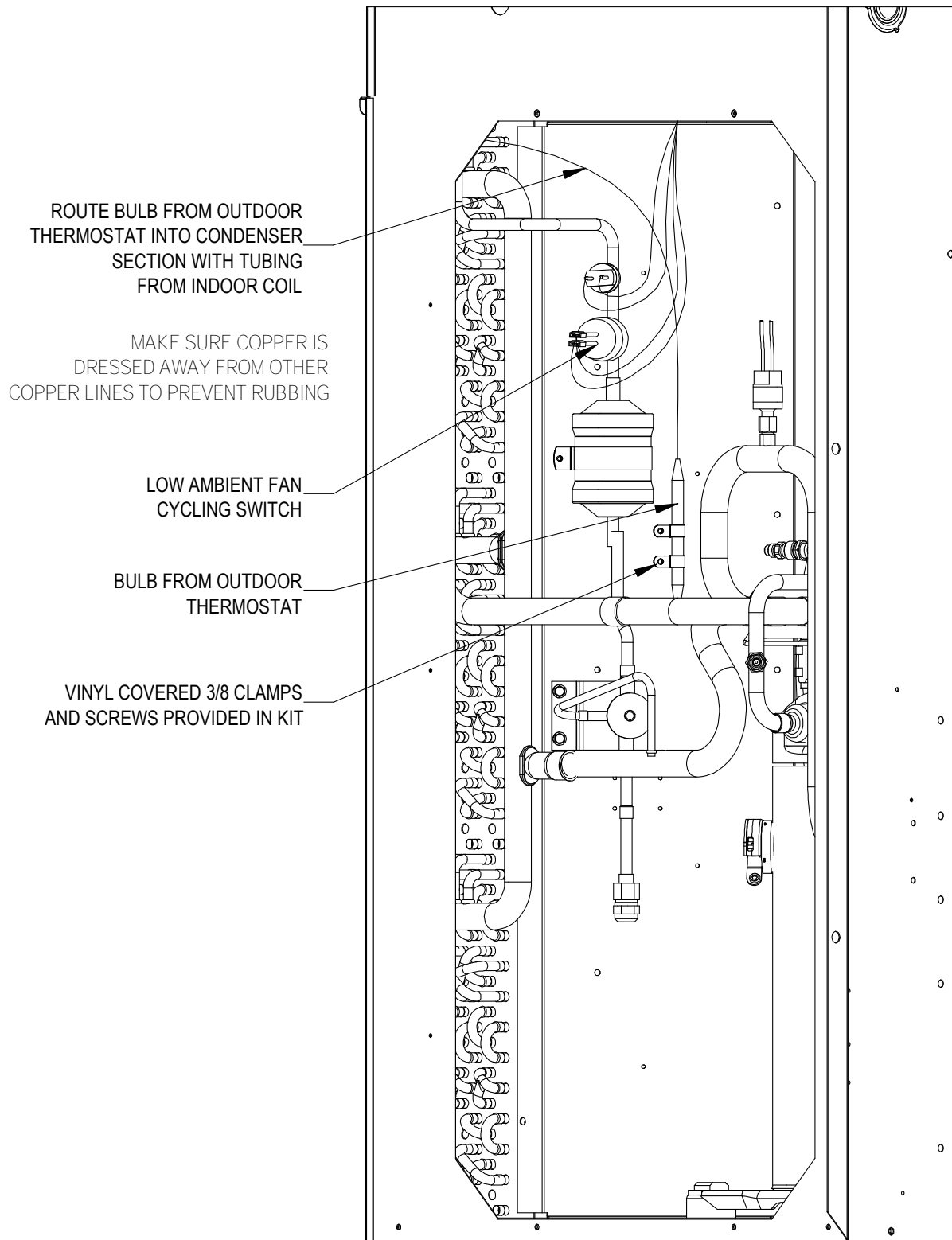
FIGURE 2 Mounting Outdoor Thermostat Bulb and/or Low Ambient Fan Cycling Switch (as applicable)
