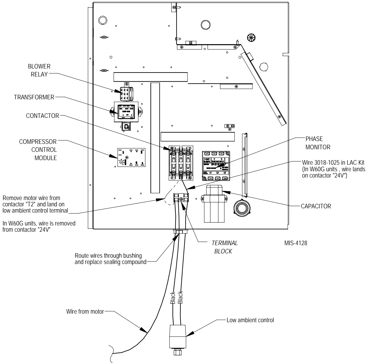
FIGURE 1 Control Panel
