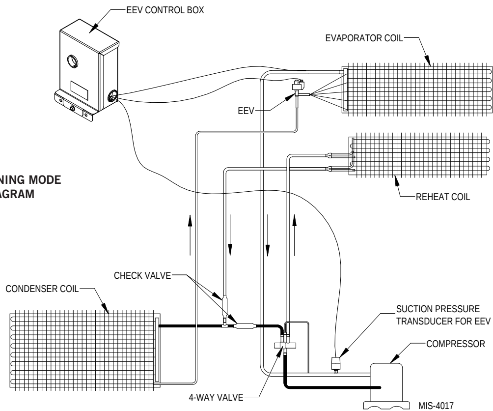
FIGURE 1 Circuit Diagrams
