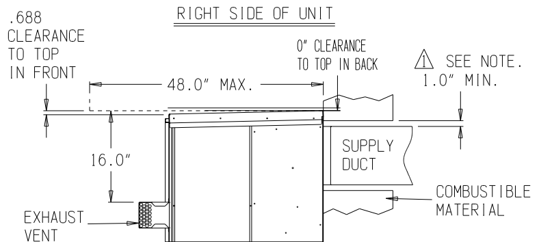
FIGURE 1 COMBUSTIBLE CLEARANCE
