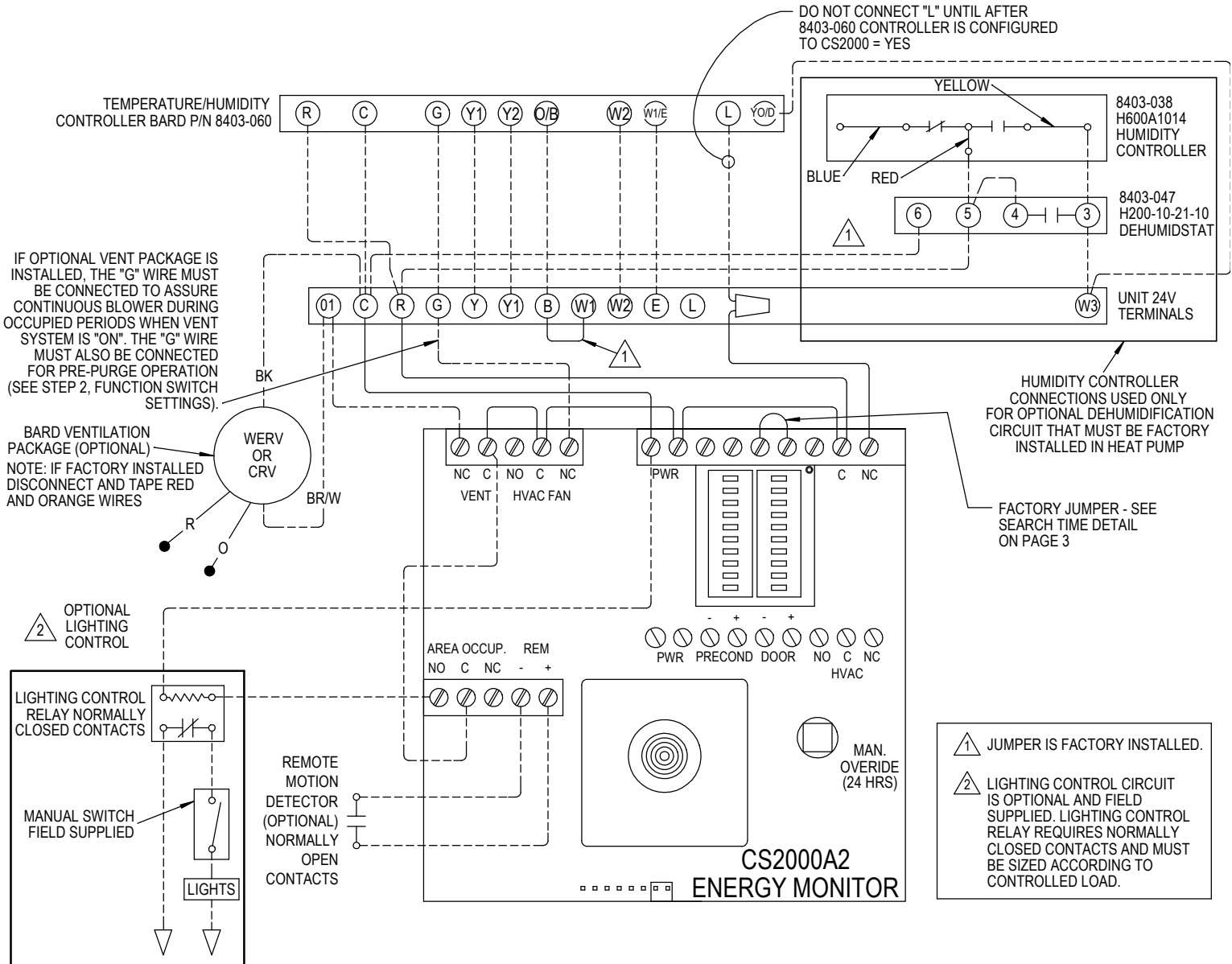
Figure 7 HP WITH CS2000 TH/SH HEAT PUMP CONNECTION DIAGRAM
