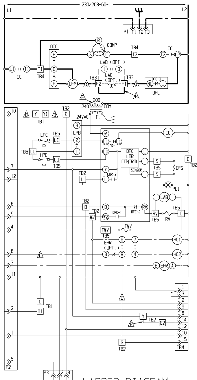
LADDER DIAGRAM
