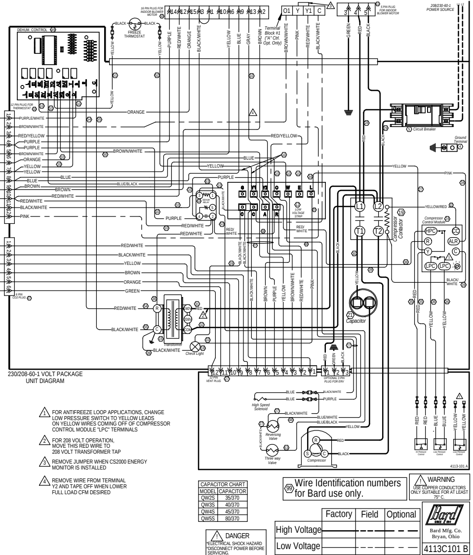
COMPOSITE WIRING DIAGRAM 230/208-60-1
