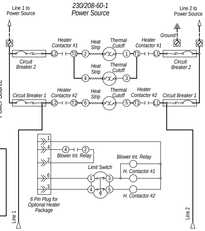
Ladder Diagram
