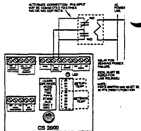
Figure 12 Connect the power-fail-sense input to either N/C or N/O contacts of a line powered relay.
