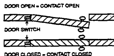
Figure 13 Required Door Switch Logic
