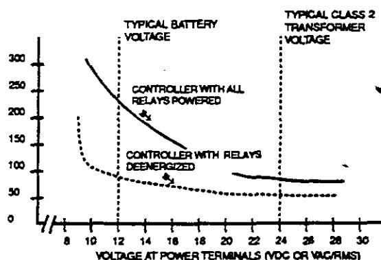
Figure 11 CS 2000's Current Draw Varies with Applied Voltage
