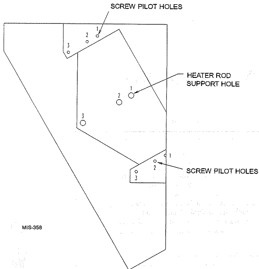
FIGURE 3 HOLES FOR HEATER ROD SUPPORT AND MOUNTING
