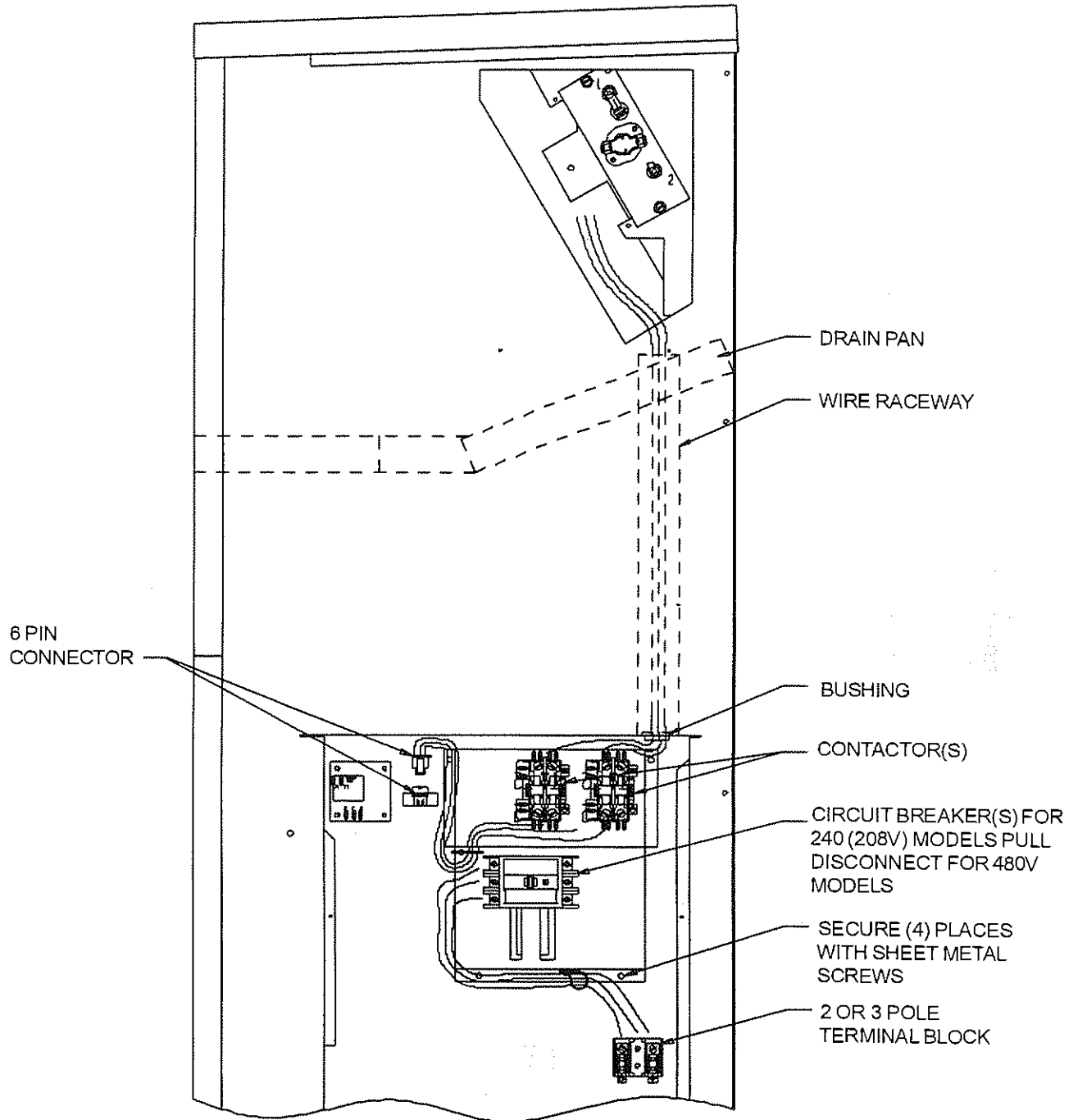
FIGURE 5 WIRE ROUTING
