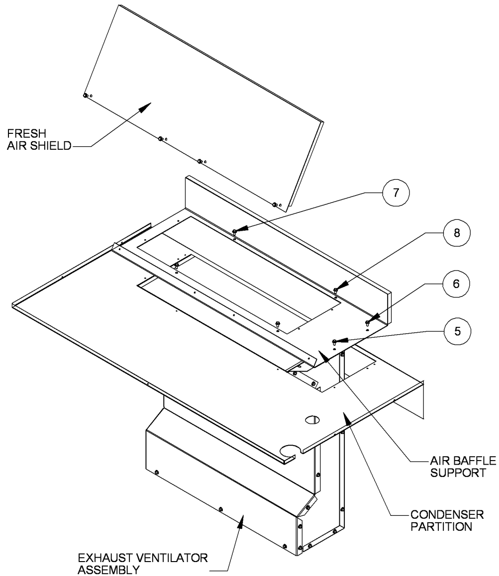
FIGURE 2 ASSEMBLY OF EXHAUST VENTILATOR AND AIR BAFFLE SUPPORT
