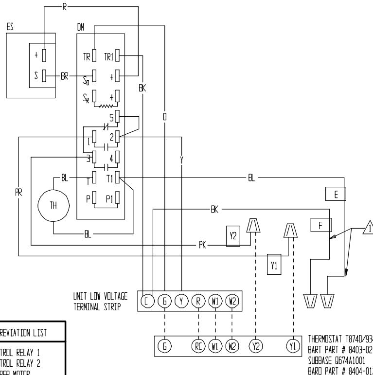
AIR CONDITIONER CONNECTION DIAGRAM
