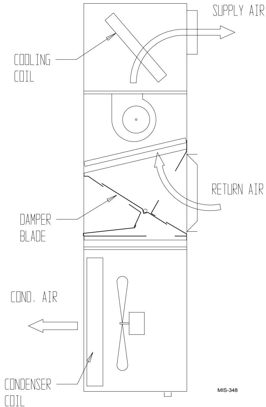
FIGURE 7 MECHANICAL COOLING OPERATION
