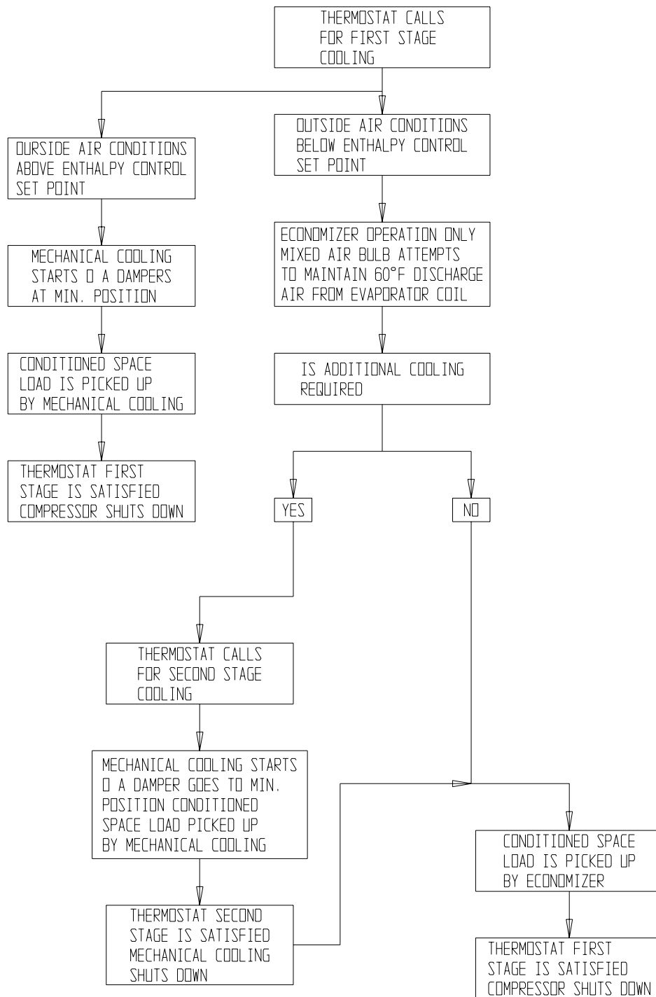
FIGURE 8 ECONOMIZER OPERATION FOR SINGLE COMPRESSOR UNIT
