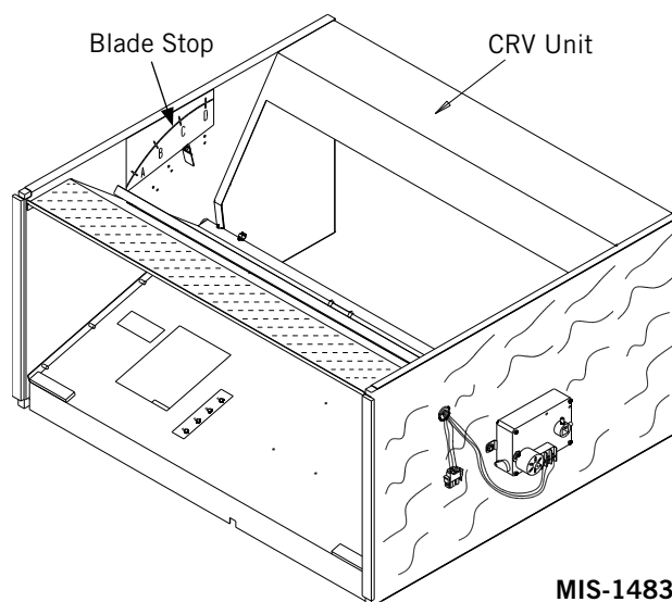
FIGURE 6 Locating Blade Stop
