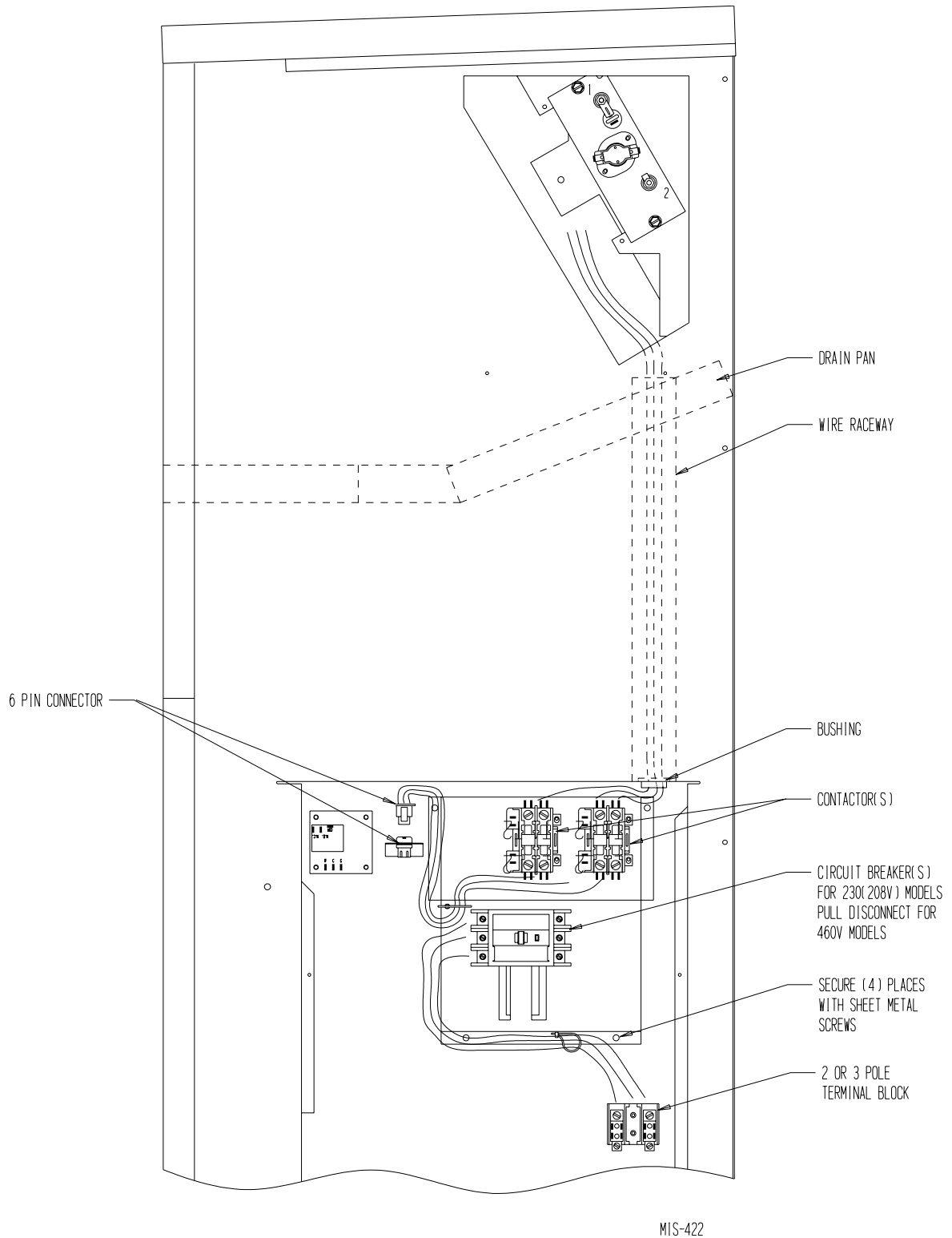
FIGURE 5 INSTALLING HEATER BASE AND CONNECTING
