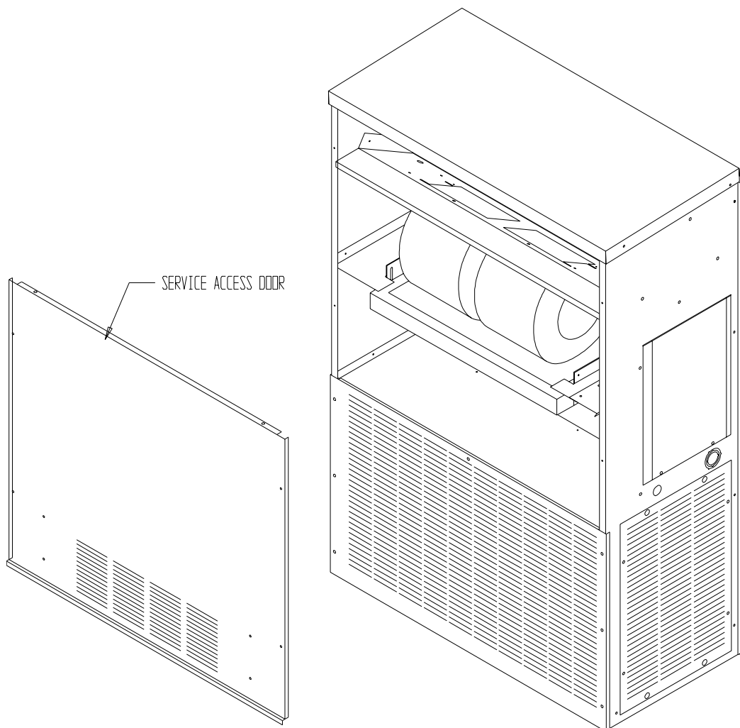
FIGURE 1 REMOVE SERVICE ACCESS PANEL
