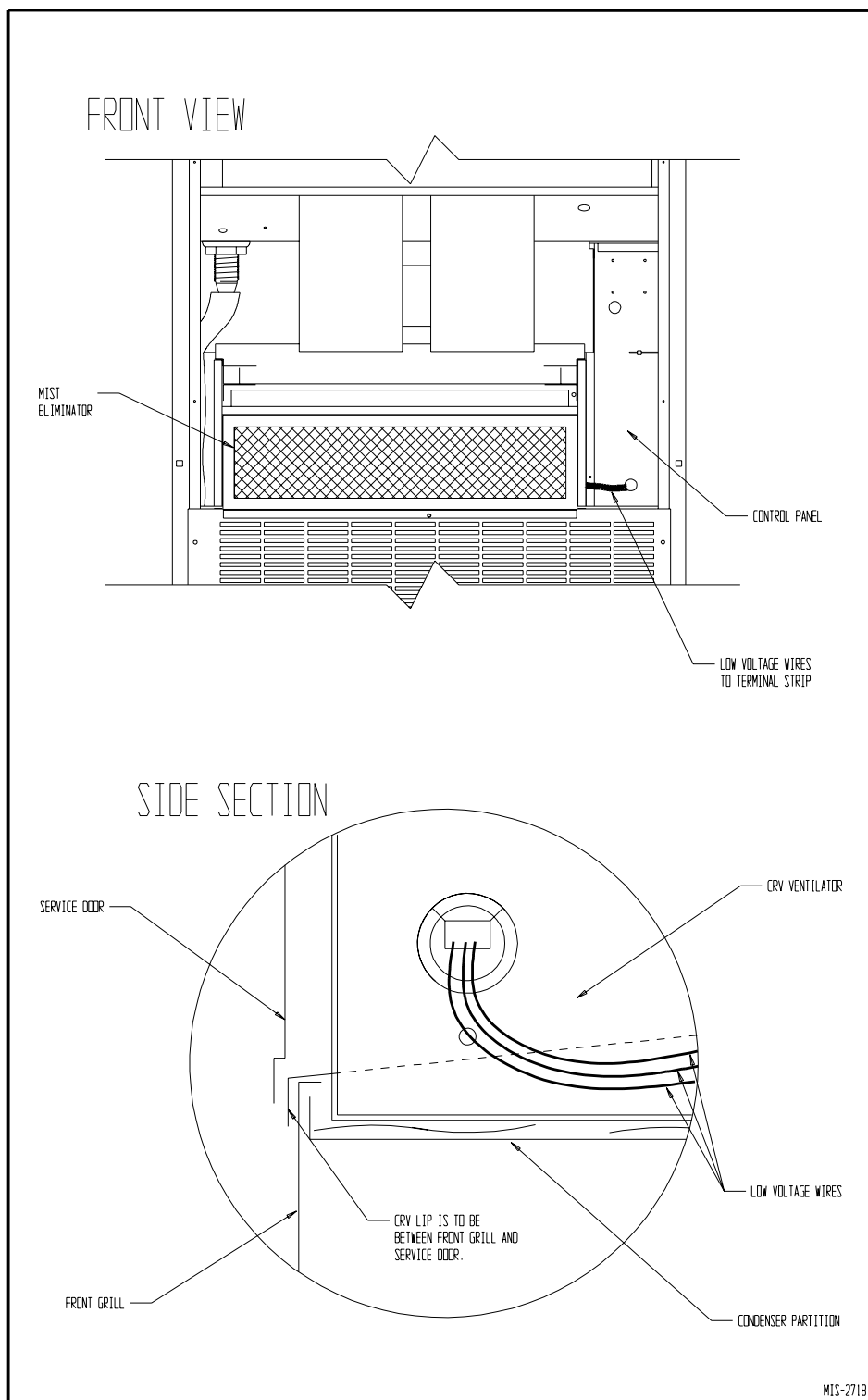
FIGURE 3 INSTALLING VENTILATOR IN UNIT
