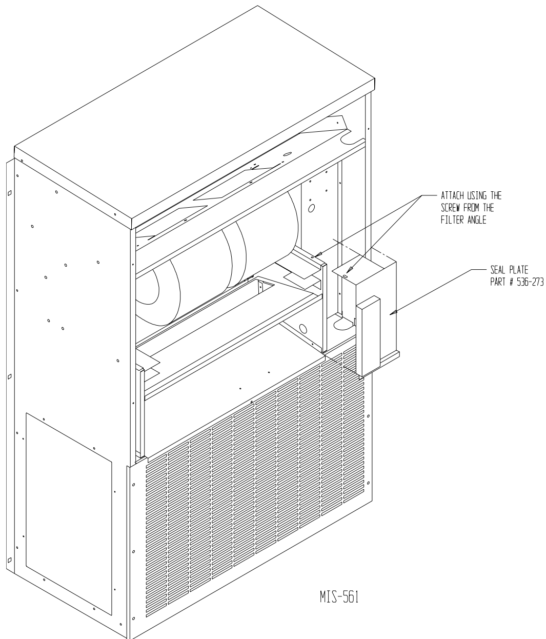
FIGURE 4 ATTACHING SEAL PLATE
