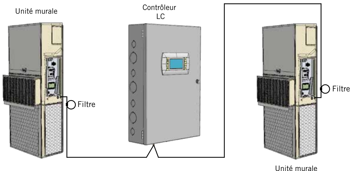
FIGURE 1.7 Câblage de communication (liaison alternative)
